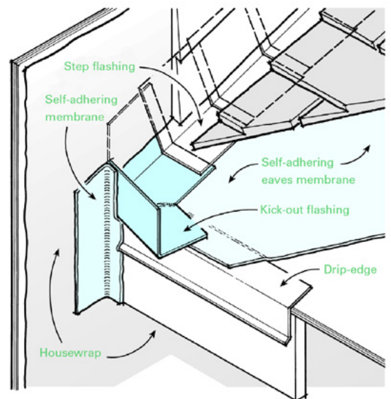
Kick-out and step flashing detail
