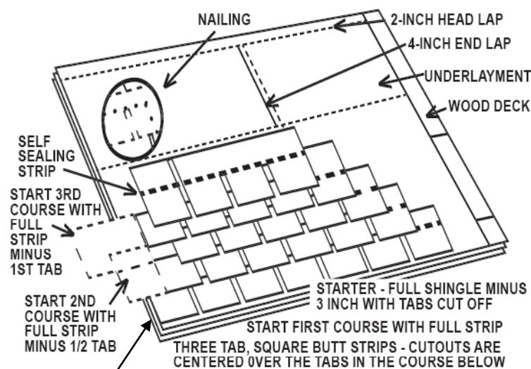
Shingle installation detail
